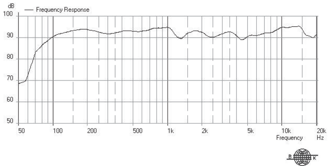
Unprocessed Anechoic Frequency Response, 1 watt @ 1 metre
